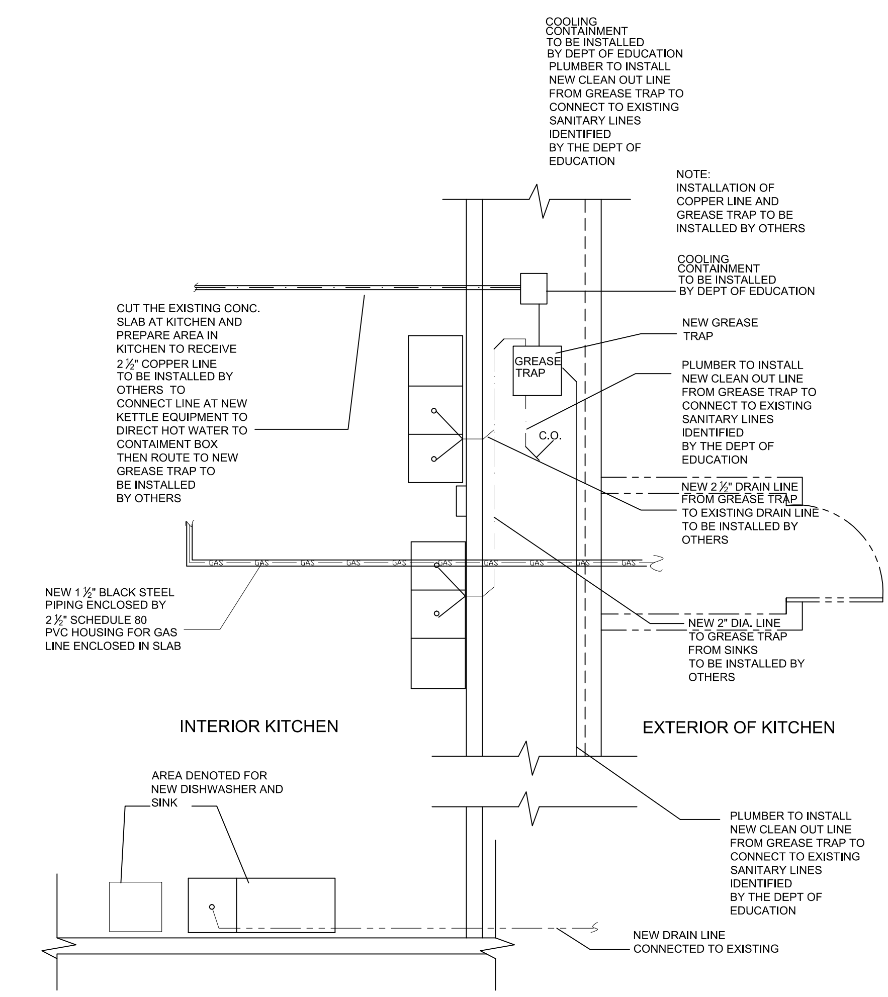
PIPING DIAGRAM
