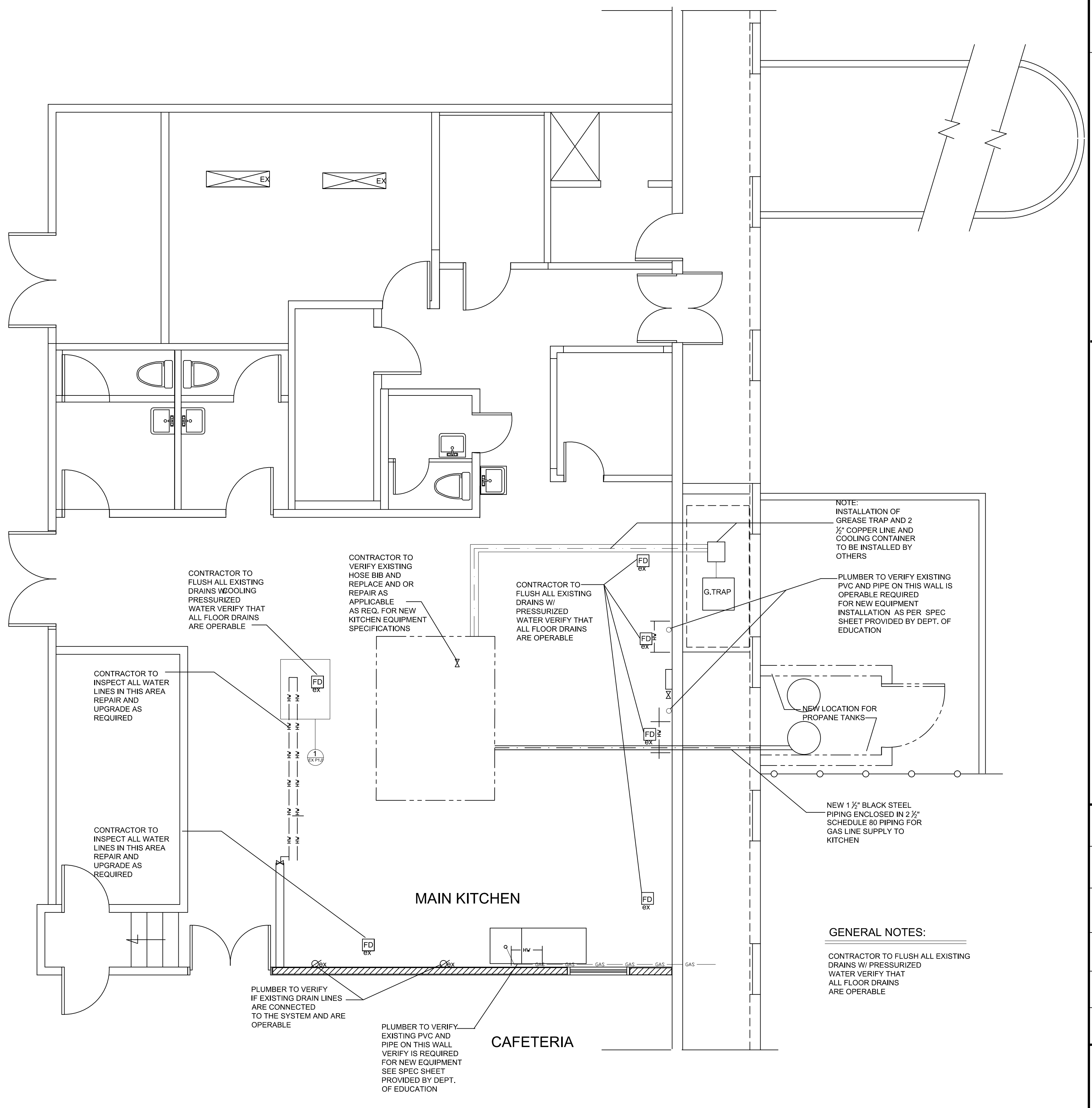
EXISTING PLUMBING LAYOUT
