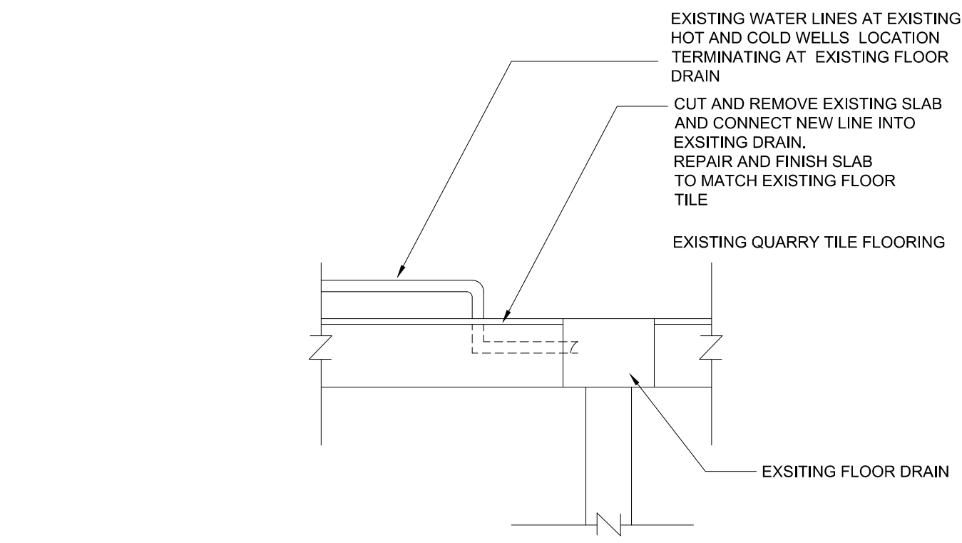
WATER LINE DETAIL ENCASEMENT @ HOT AND COLD WELL LOCATION SERVICE LINES
