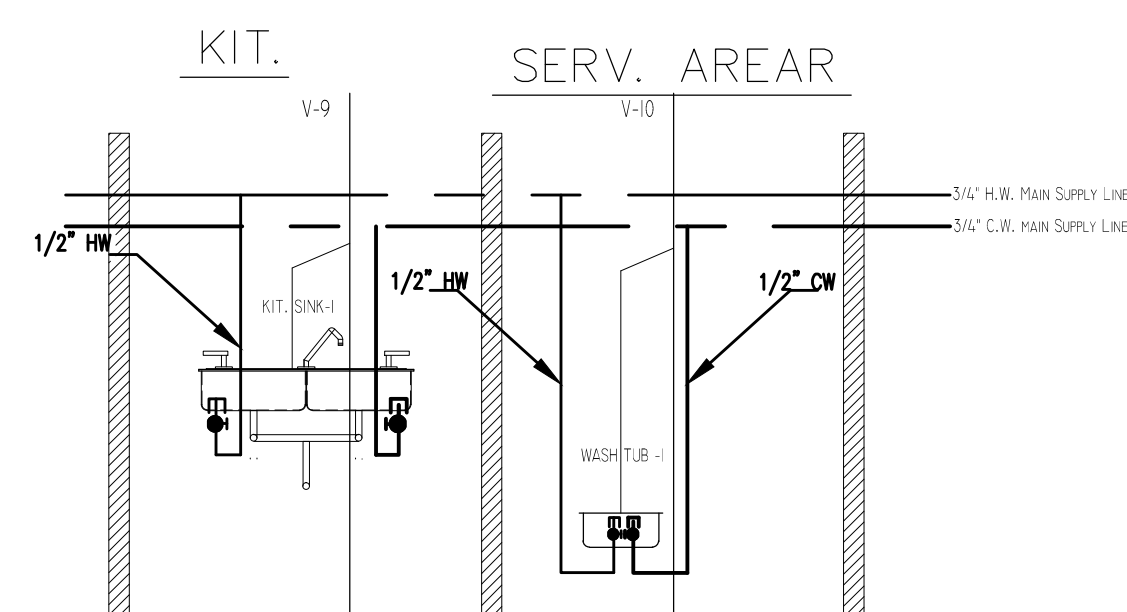
CONCESSION BUILDING HOT AND COLD WATER RISER DIAG.
