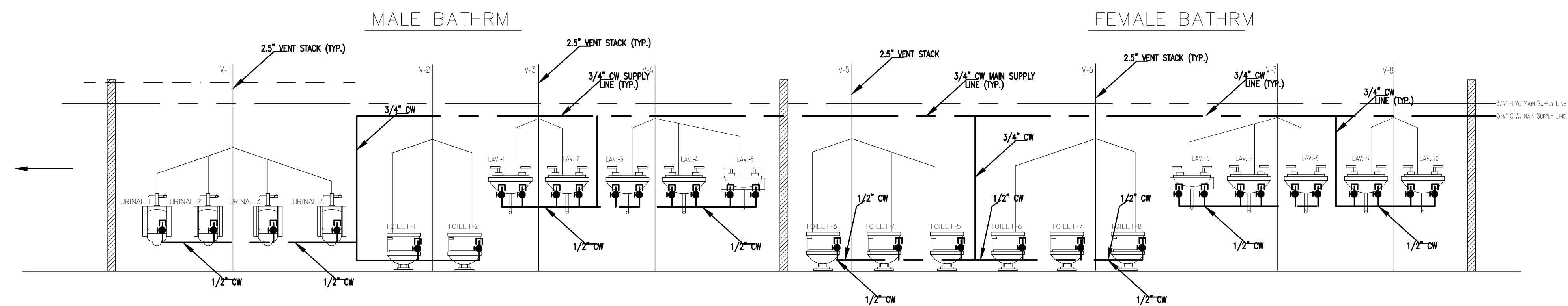
BATHROOM BUILDING HOT AND COLD WATER RISER DIAG.
