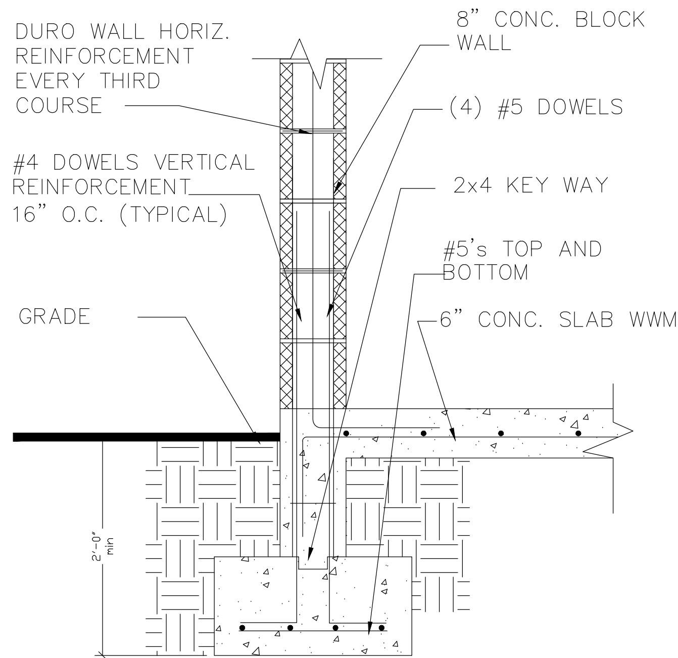
2 FOOTING DETAIL Scale: 1" = 1'-0"
