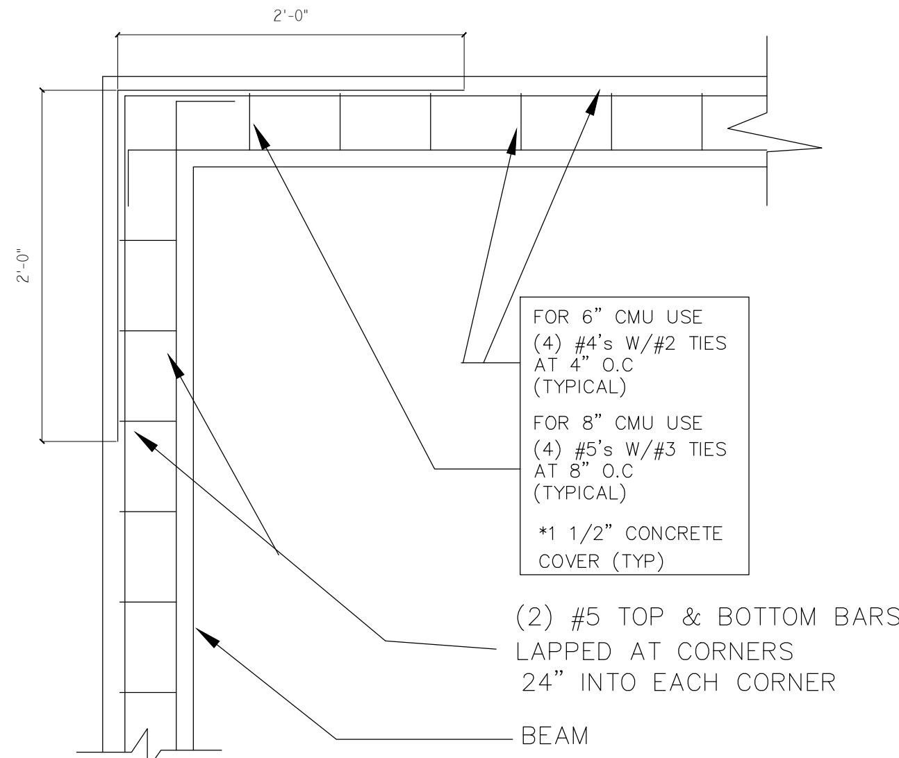
4 BOND BEAM DETAIL @ CORNER Scale: 1" = 1'-0"
