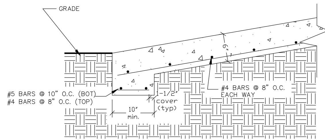
1 RAMP DETAIL Scale: 3/4" = 1'-0"
