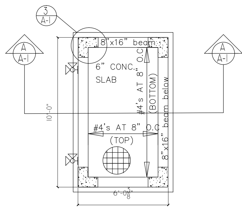
CONC. ROOF PLAN Scale: 1/4" = 1'-0"
