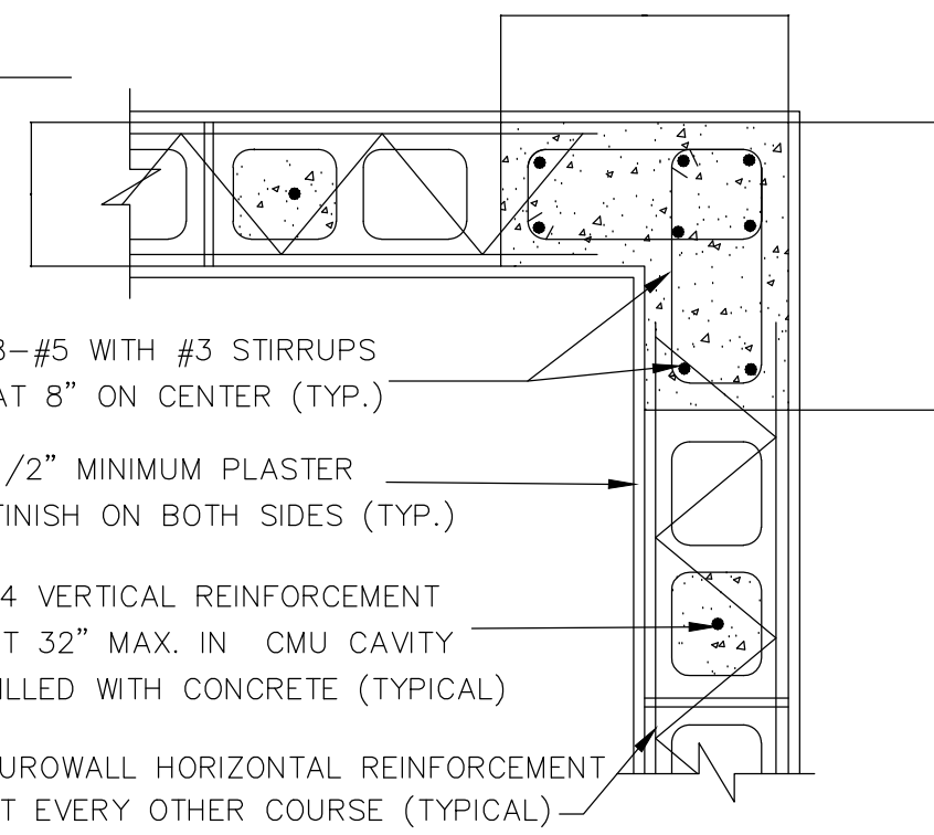
3 CONCRETE COLUMN CORNER DETAIL Scale: 1" = 1'-0"
