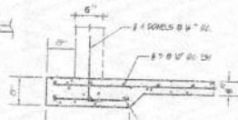
FOOTING DETAIL-A
