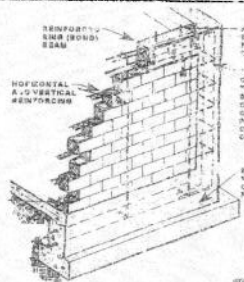
TYPICAL MASONRY
