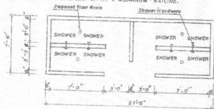
DIMENSIONAL FLOOR PLAN 50' 1/4\"/>
