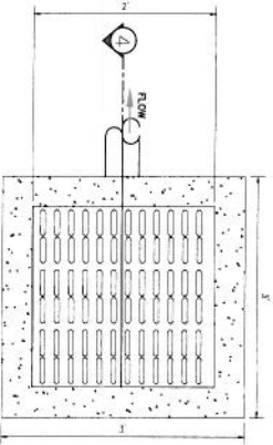
TYPICAL DRAINAGE INLET
